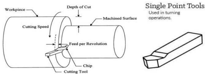
Fig.1: Turning Process
