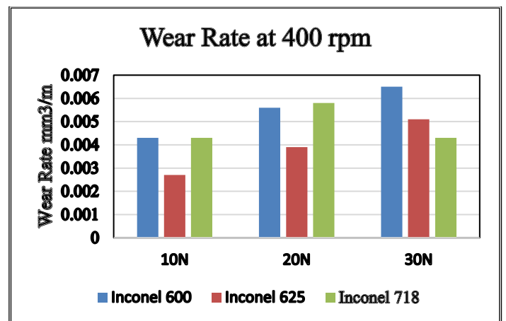
Figure 5 Wear rate at 400 rpm
