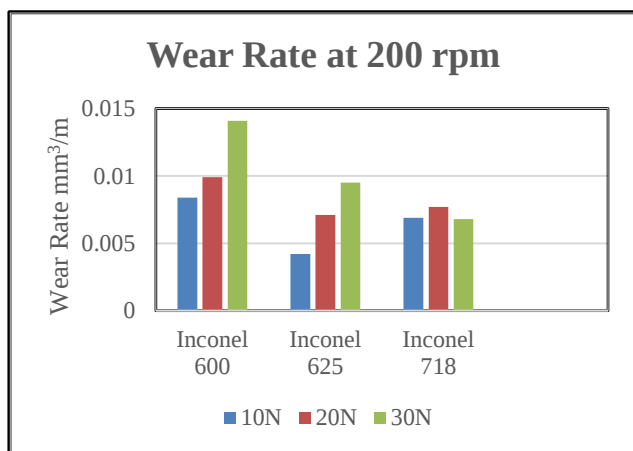
Figure 3. Wear rate at 200 rpm
