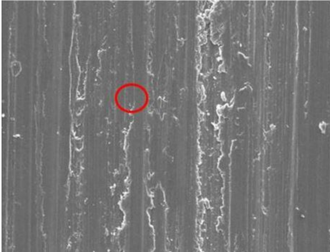
Figure 10 worn-out surfaces for the Inconel 625- Cr 3 C 2 -NiCr coatings for the speed of 300 rpm and load of 20N
