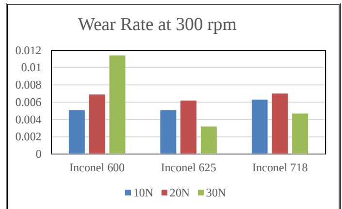
Figure 4 Wear rate at 300 rpm
