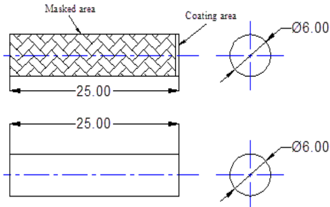
Figure 1 Dimension of Coated Inconel Wear Specimen
