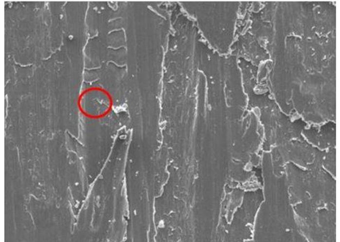
Figure 8 worn-out surfaces for the Inconel 600- \text{Cr}_3\text{C}_2 -NiCr coatings for the speed of 400 rpm and load of 20N
