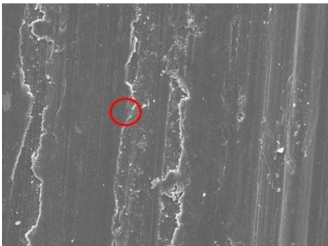
Figure 13 worn-out surfaces for the Inconel 718-Cr 3 C 2 -NiCr coatings for the speed of 300 rpm and load of 20N
