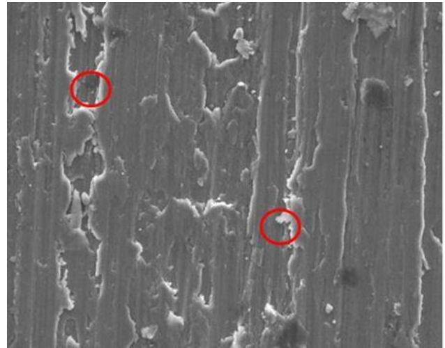
Figure 11 worn-out surfaces for the Inconel 625- Cr 3 C 2 -NiCr coatings for the speed of 400 rpm and load of 20N
