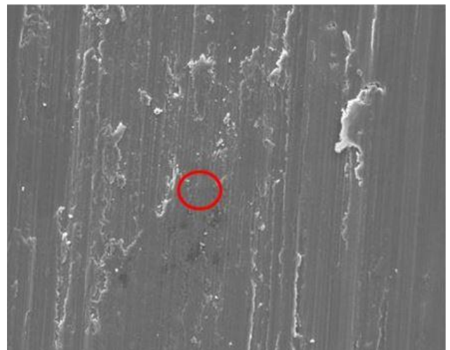
Figure 7 worn-out surfaces for the Inconel 600- \text{Cr}_3\text{C}_2 -NiCr coatings for the speed of 300 rpm and load of 20N
