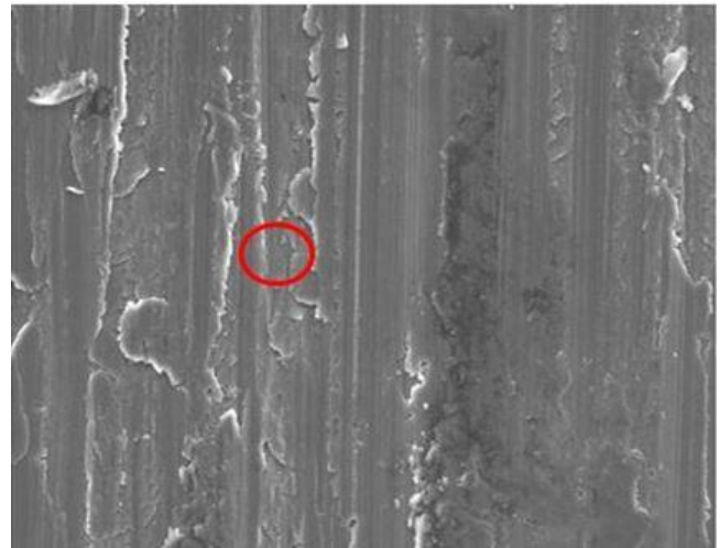
Figure 14 worn-out surfaces for the Inconel 718-Cr 3 C 2 -NiCr coatings for the speed of 400 rpm and load of 20
