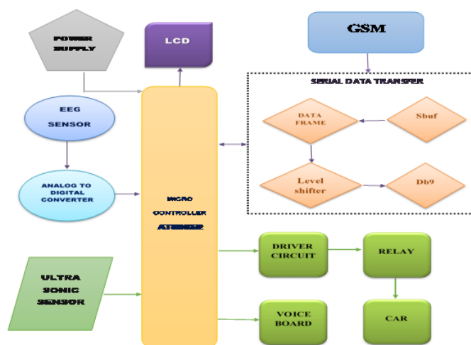
Fig 1: Block diagram of mental fatigue detection
