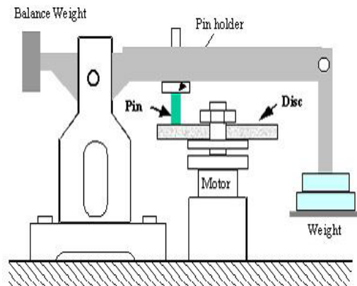
Figure 4. Pin-on-disc apparatus
