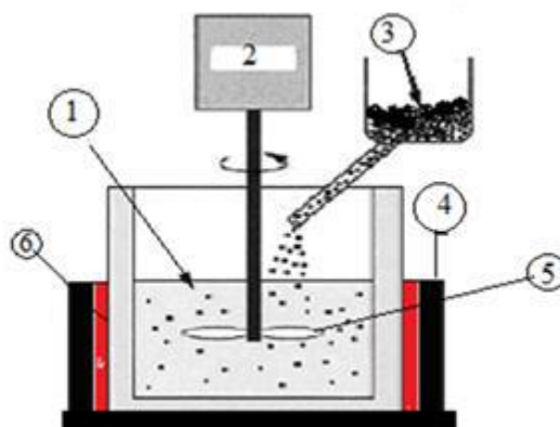
Figure 2. Stir casting setup. 1. Aluminium liquid, 2. Electric motor, 3. Marula seed cake, 4. Insulated board, 5. Blades, 6. Crucible
