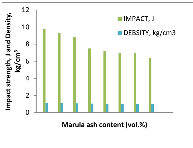
Figure 7. Effect of MSC on the impact strength and density of Al6061.
