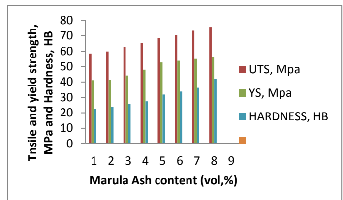
Figure 6. Effect of MSC on the strength and hardness of Al6061
